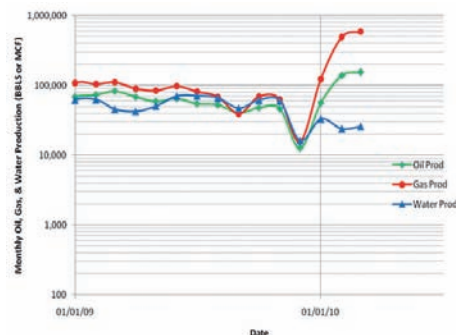
MC711 #AST1 monthly production chart.
